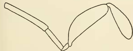
FIG. 44.—MUNNOPSIS LATIFRONS. SEVENTH LEG. \times 4\frac{2}{3} .
